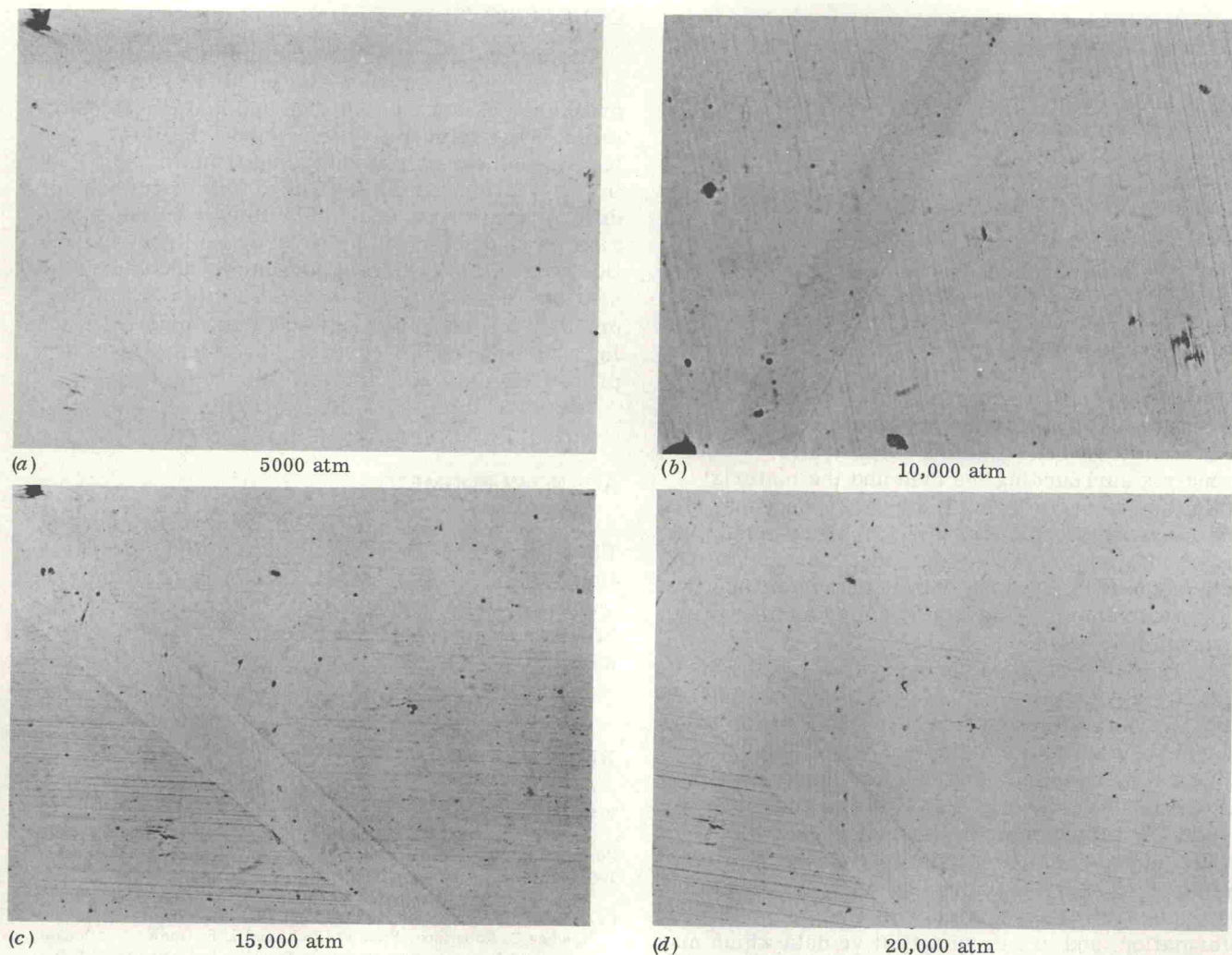
Fig. 12—Mechanically twinned area subsequently subjected to extreme pressure. X100. Enlarged approximately 5 pct for reproduction.
